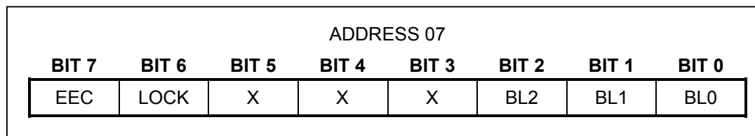
Figure 13. EEPROM Register Format
